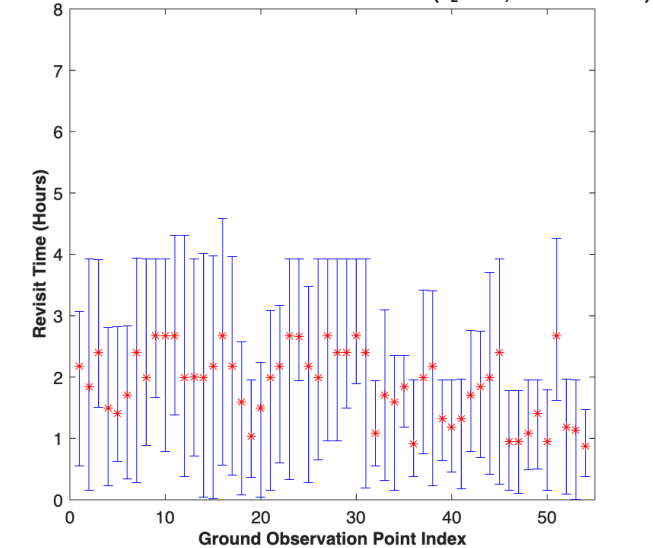
Worldwide Ground Points Revisit Time Result ( L_2 BCD, \tau = 1000 sec)
