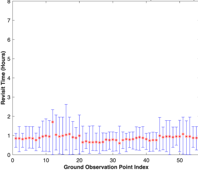
Worldwide Ground Points Revisit Time Result (Unconstrained)
