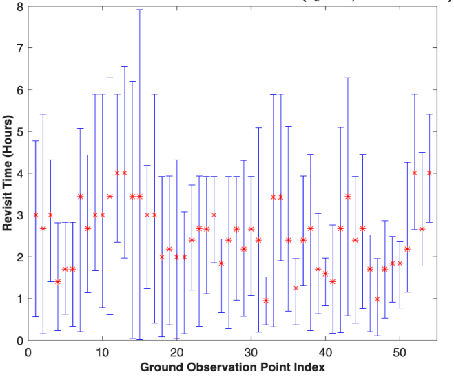
Worldwide Ground Points Revisit Time Result ( L_2 BCD, \tau = 4000 sec)
